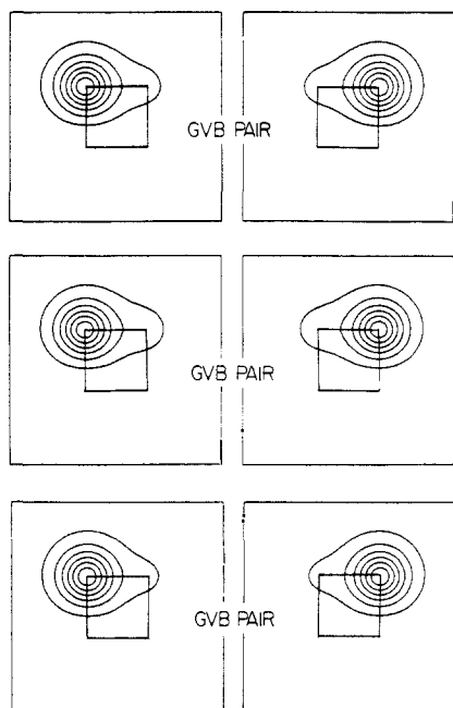
Figure 4. The GVB and GRVB orbitals for one bond pair of singlet cyclobutadiene: top, GVB(2/4); middle, GRVB(2/4) ^1B_{1g} (resonant) state; bottom, GRVB(2/4) ^1A_{1g} (antiresonant) state. Only one of the two (equivalent) bond pairs is shown in each case. All orbitals are plotted in a plane to 0.5 Å above, and parallel to, the plane of the molecule. The projected positions of the atoms are included on the plots for clarity, and the contours range from -1.0 to 1.0 au by increments of 0.05, with negative contours represented by dotted lines.
