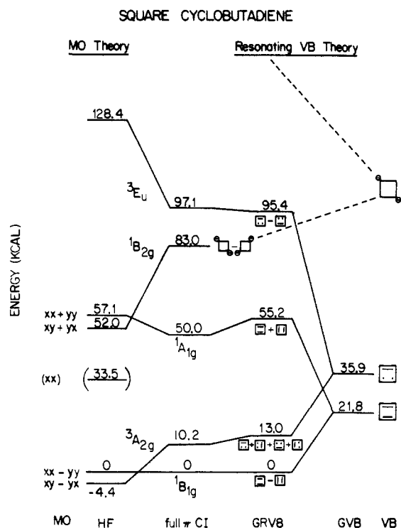
Figure 3. Quantitative comparison of MO theory and resonating VB theory. The total energies for the ^1B_{1g} state are the following: HF, -153.58584; GRVB, -153.65295; and full \pi CI, -153.65783. The GRVB and \pi CI wave functions use the same frozen \sigma core, while the core orbitals for the HF wave functions are completely relaxed for each state.
